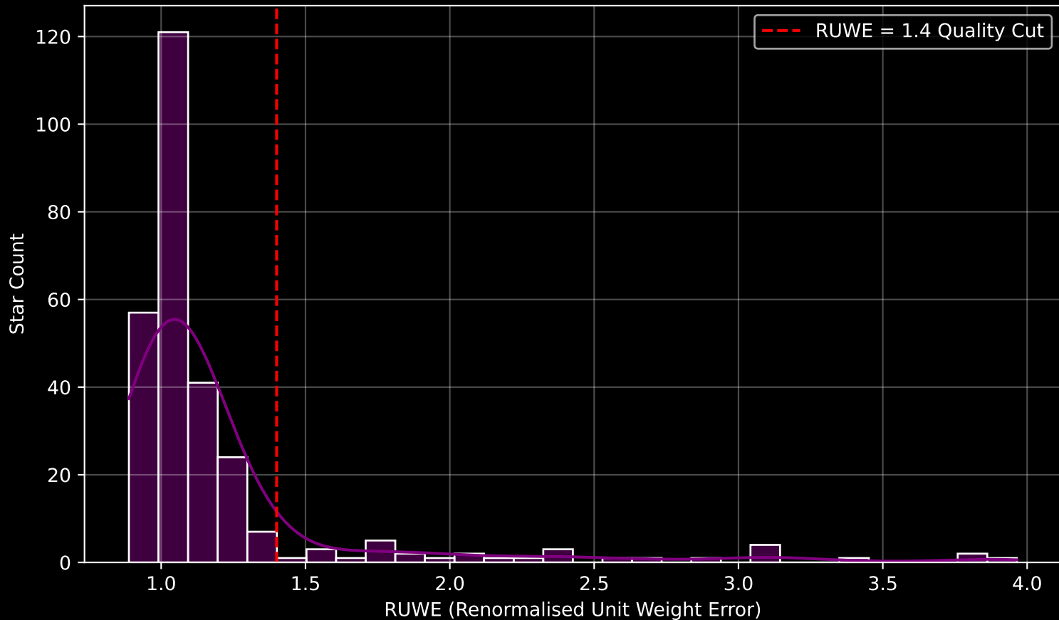
GALAH DR4 Field [7041] RUWE Distribution (n= 281)
