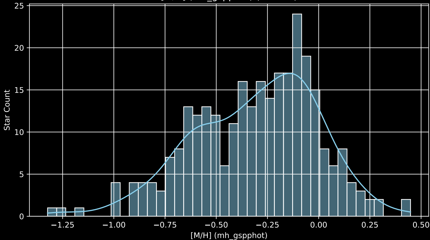
GALAH DR4 Field: [7041] [M/H] (mh_gspphot) (n= 290)
