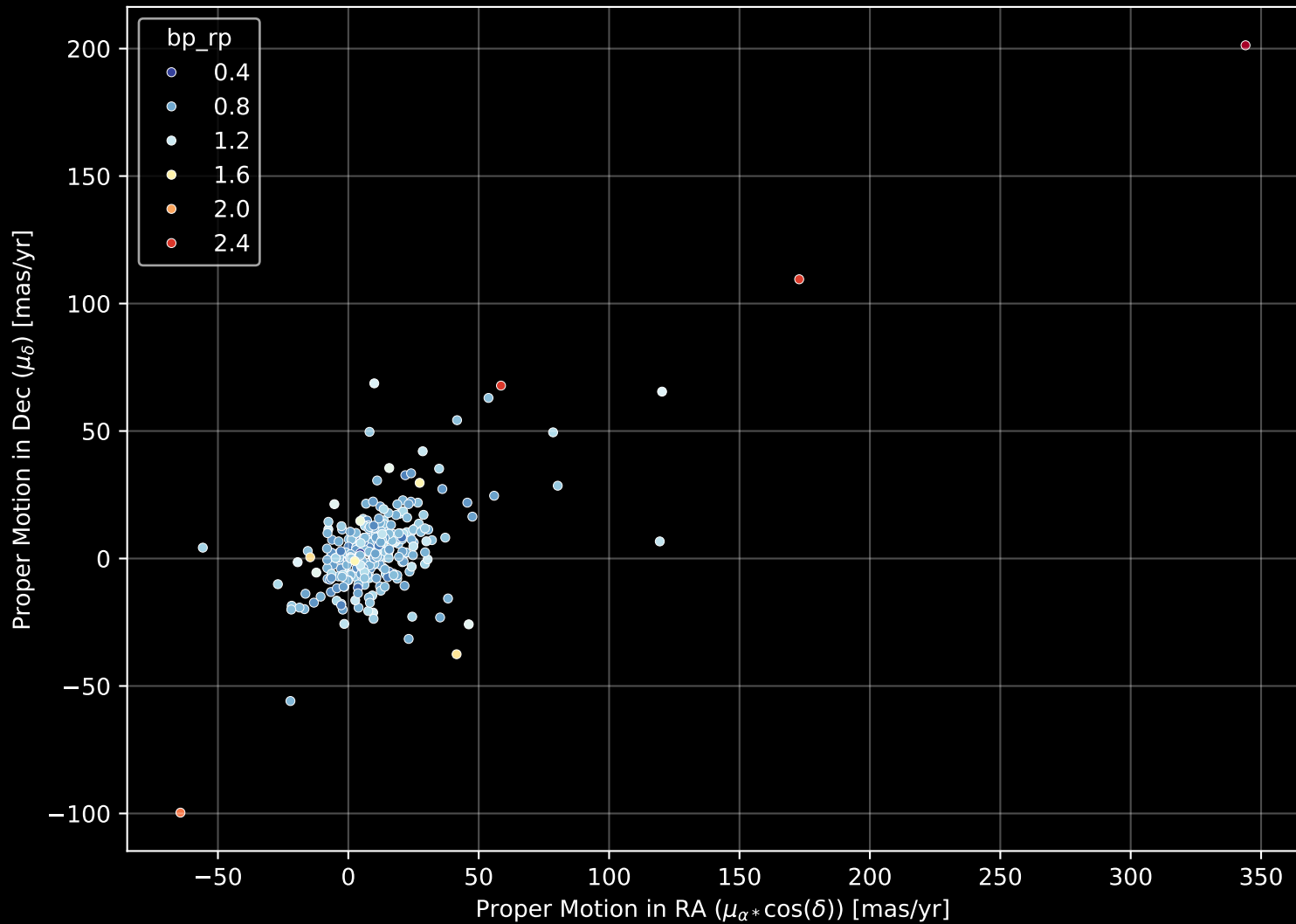
GALAH DR4 Field: [7041] Proper Motion Diagram (n= 291)
