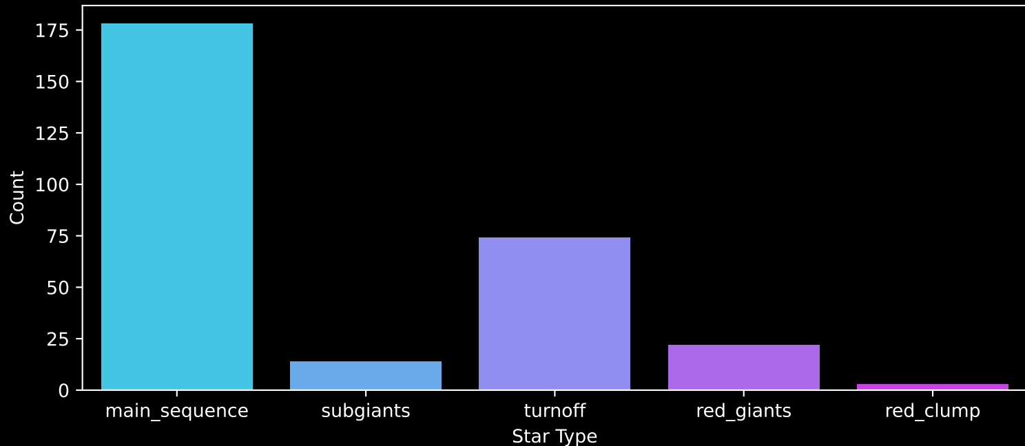
GALAH DR4 Field: [7041] Count plot of Star Type
